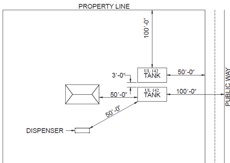
Commentary Figure 2306.2.3(6) ALL OTHER ABOVE-GROUND STORAGE TANKS STORING CLASS II OR III LIQUIDS ONLY
