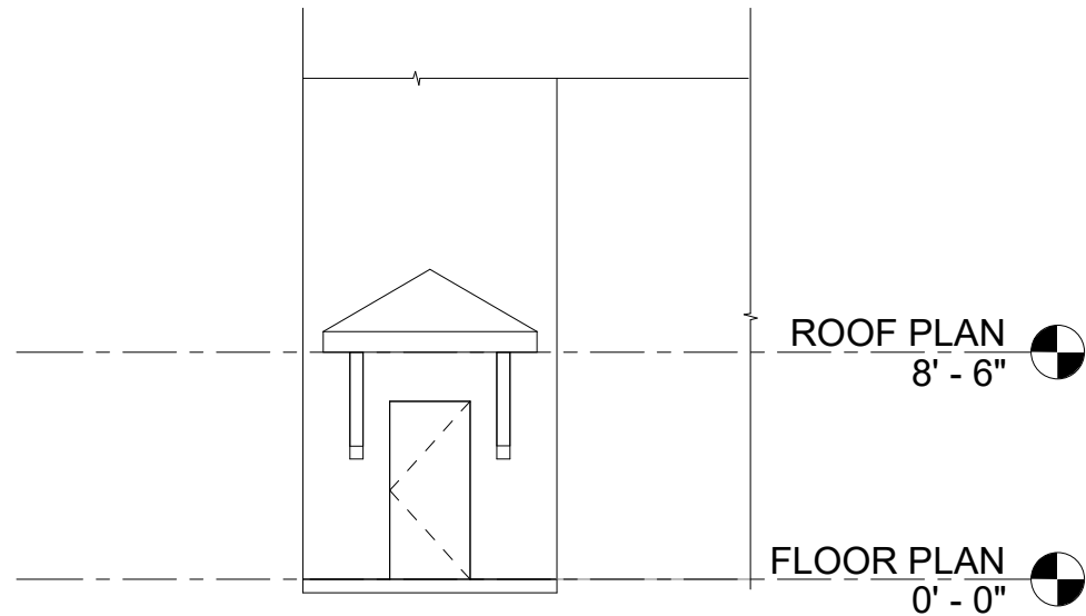
3 SOUTH ELEVATION 1/8" = 1'-0"
