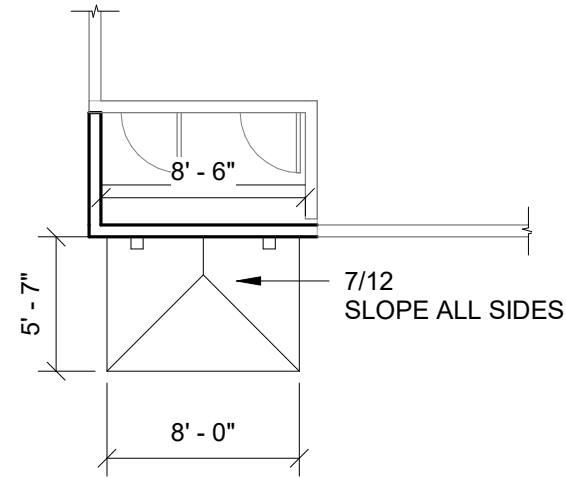
2 ROOF PLAN 1/8" = 1'-0"
