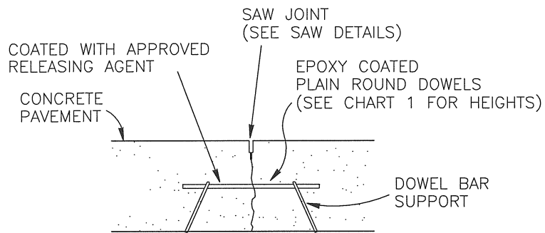
SECTION A-A DOWEL ASSEMBLY
