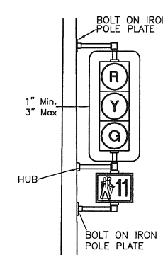
TYPE IV POST MOUNTED-VEHICULAR POST MOUNTED-PEDESTRIAN
