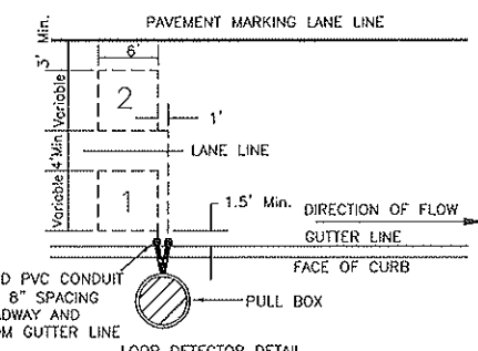
LOOP DETECTOR DETAIL (PASSAGE OR CALLING)
