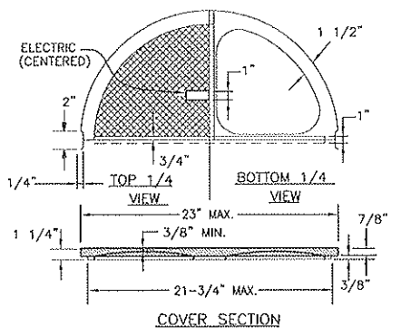
FRAME AND COVER CASTING
