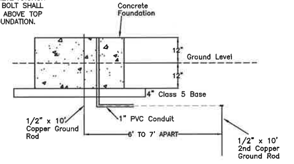
COMBO PAD MOUNTED FEED POINT
