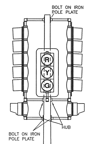
TYPE VIII-17.5' HEIGHT PEDESTAL MOUNTED-VEHICULAR PEDESTAL MOUNTED-PEDESTRIAN
