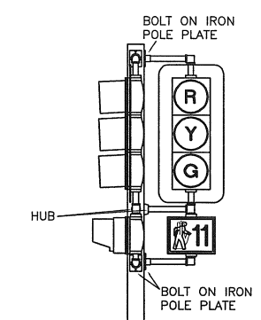
TYPE V-15' HEIGHT PEDESTAL MOUNTED-VEHICULAR AND PEDESTRIAN HEADS
