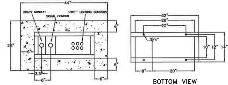
BASE DETAIL
