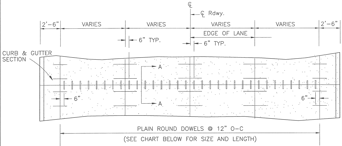
TRANSVERSE CONTRACTION JOINT DOWEL ASSEMBLY
