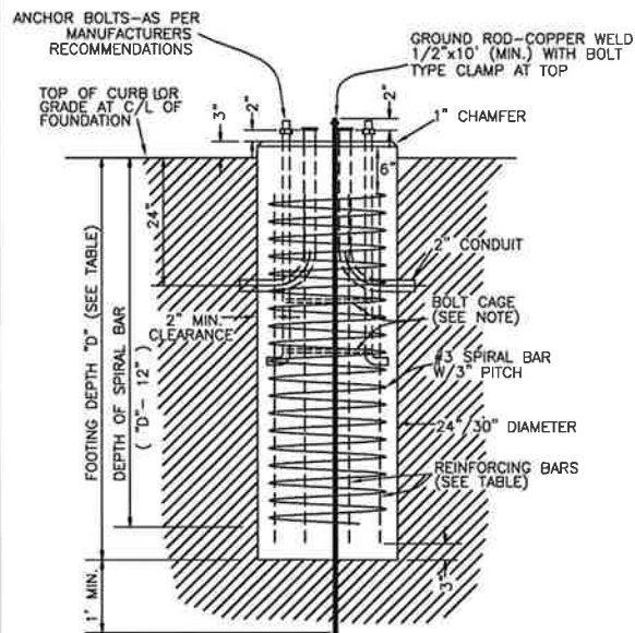
ELEVATION 24" DIA. FOUNDATION TYPE V PEDESTRIAN FLASHER FOUNDATIONS
