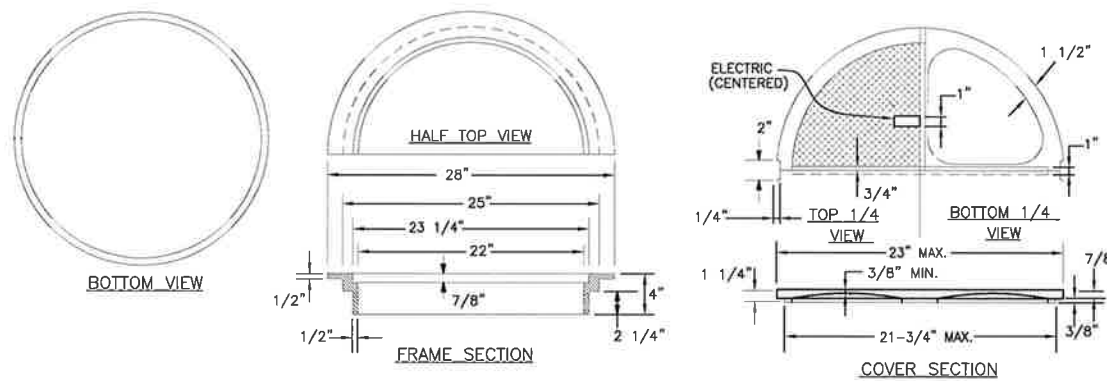
TYPE V PED. FLASHER MOUNTED PUSH BUTTON DETECTOR
