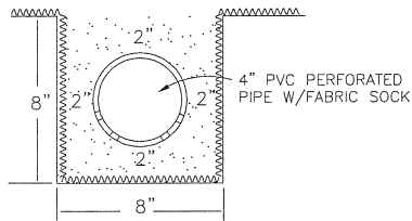
TRENCH DETAIL
