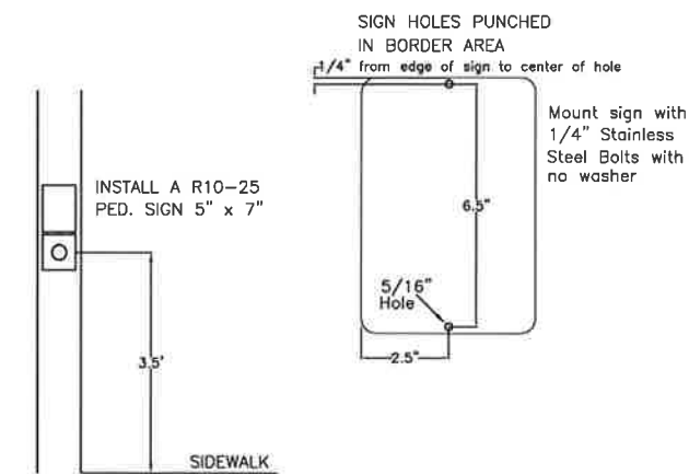
TYPE V PED. FLASHER MOUNTED PUSH BUTTON DETECTOR
