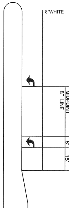
TYPICAL TURNBAY-NO STOP BAR STOP AT END OF ISLAND
