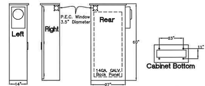
POLE MOUNTED FEED POINT
