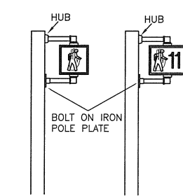
TYPE V-10' HEIGHT PEDESTAL MOUNTED-PEDESTRIAN
