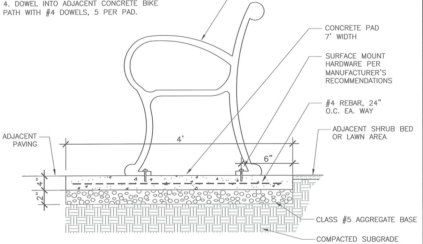
BENCH AND CONCRETE PAD DETAIL NOT TO SCALE
