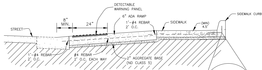
SIDEWALK REINFORCEMENT
