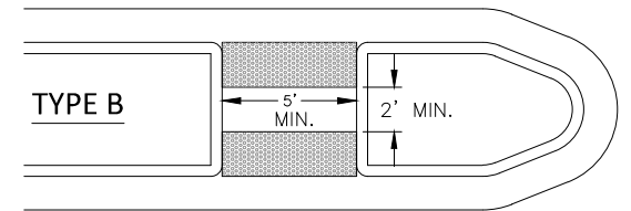
MEDIAN REFUGE ISLANDS (CUT-THROUGH)
