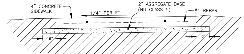
SIDEWALK CROSS-SECTION
