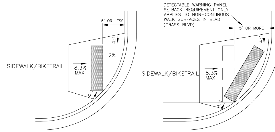
CONCRETE APRON FOR SIDEWALK/BIKETRAIL
