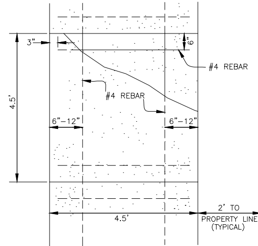
4.5' REINFORCEMENT
