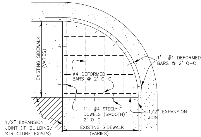
SIDEWALK REINFORCEMENT
