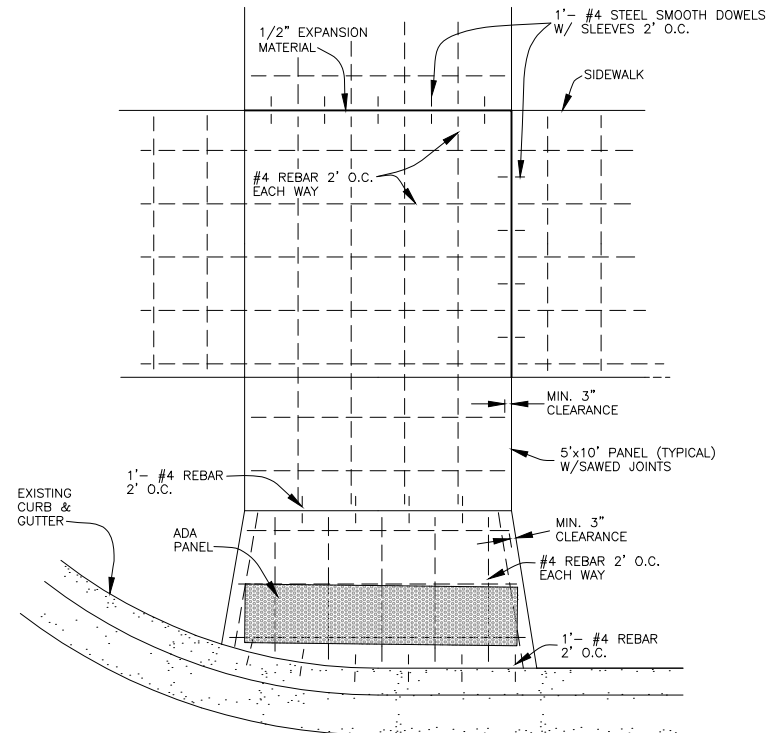
10' REINFORCEMENT
