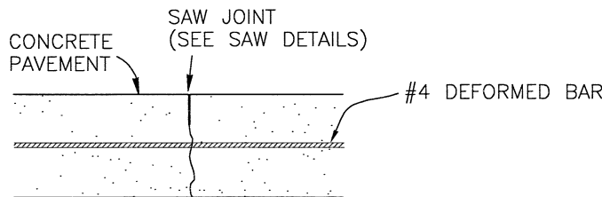
SAWED JOINT DETAIL
