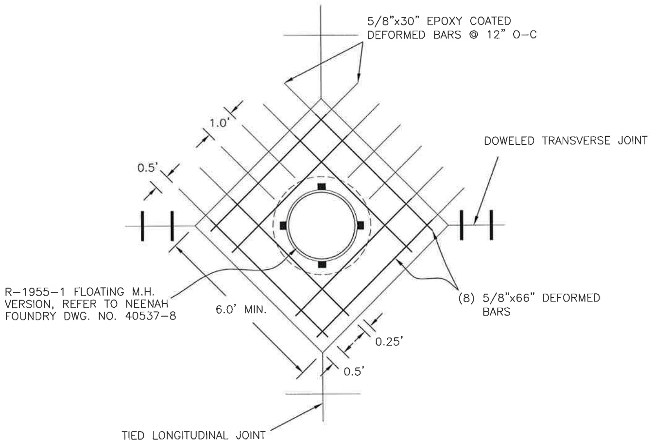
MANHOLE ISOLATION DETAIL
