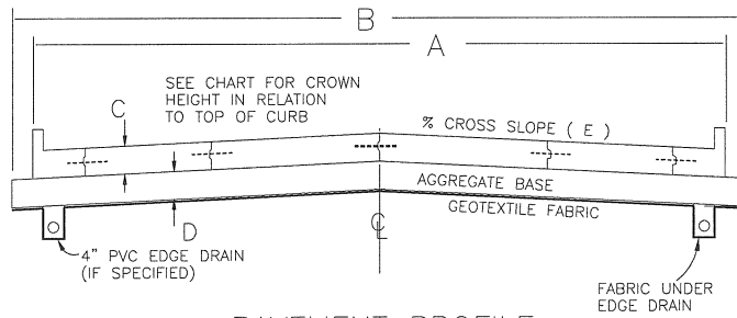
PAVEMENT PROFILE
