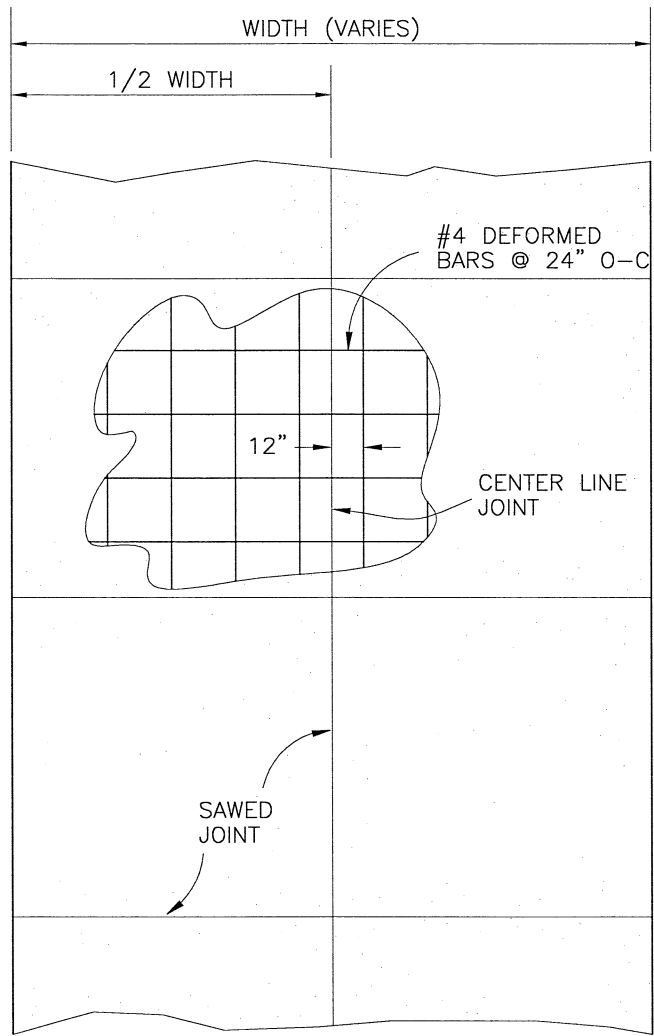
PLAN
