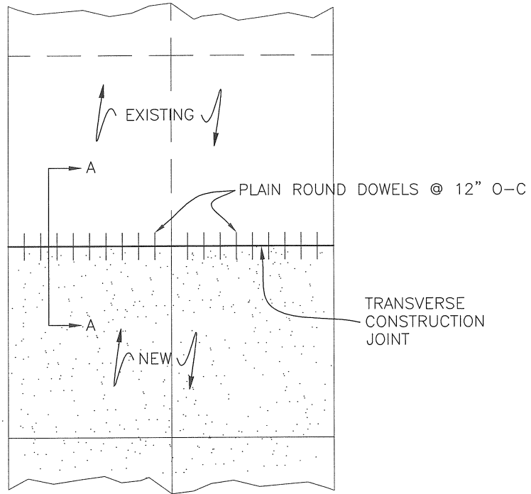
CONSTRUCTION JOINT EXISTING TO NEW CONCRETE PAVEMENT
