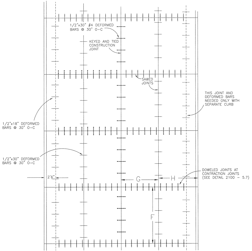
PLAN VIEW
