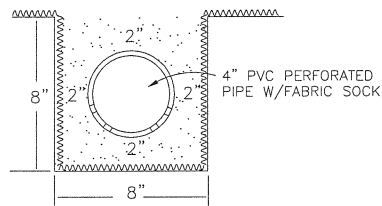
TRENCH DETAIL
