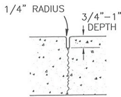
TOOLED JOINT DETAIL SECTION B-B
