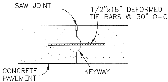
SECTION C-C LONGITUDINAL CONSTRUCTION JOINT
