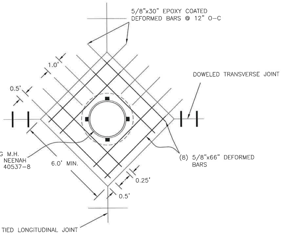
MANHOLE ISOLATION DETAIL
