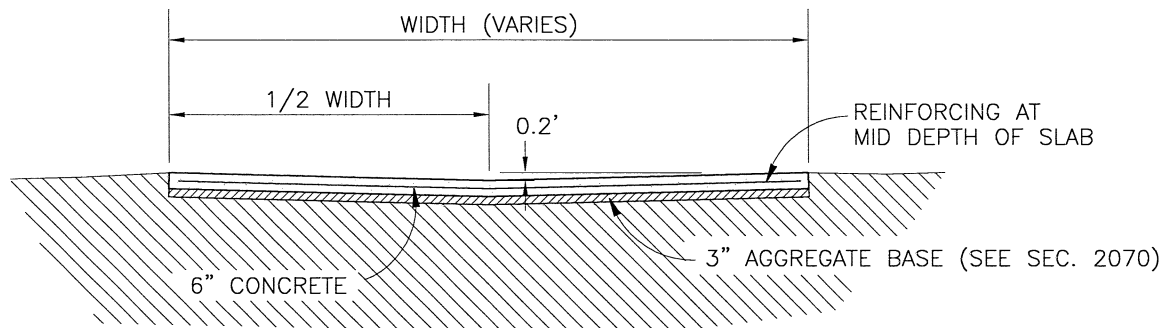
SECTION
