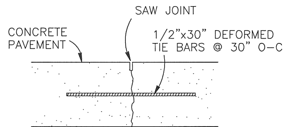
SECTION B-B SAWED LONGITUDINAL JOINT
