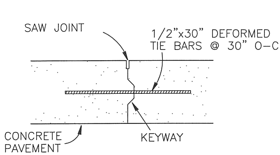
SECTION A-A LONGITUDINAL CONSTRUCTION JOINT
