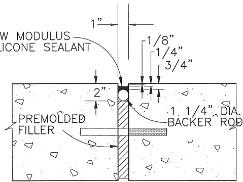
SILICONE SEAL (IF SPECIFIED)
